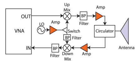
Diagram of the front end of the baseline radar system
