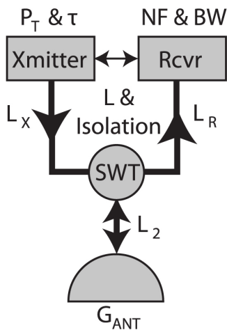
Basic radar components
