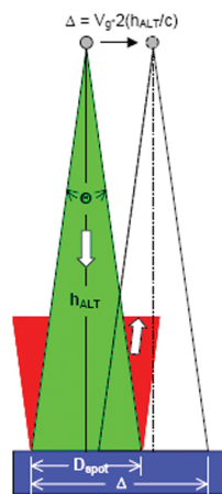
Use of pulsed radar for radiosonde observation (RAOB) measurement
