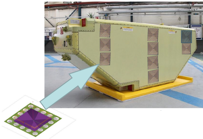
Fuel Quantity Indication System (FQIS) with SansEC sensors applied to the outside
