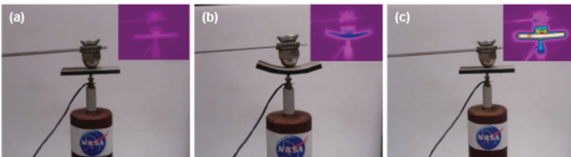
Electric field activated shape memory behavior of LaRC VSPc. (a) permanent shape, (b) programmed temporary shape, and (c) recovered permanent shape (inset: infrared images).
