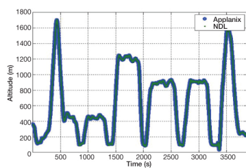
Altitude measurement from a helicopter using a Linear Frequency-Modulated Laser system (Applanix Corporation).
